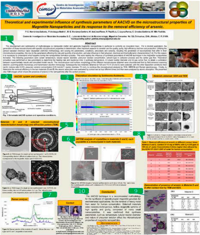
Fuente: CIMAV, Póster premiado en el Congreso ISMANAM 2014: “Theoretical and Experimental Influence of Synthesis Parameters of AACVD on the Microstructural Properties of Magnetite Nanoparticles and its Response to the Removal Efficiency of Arsenic”. Cuyos autores son: P. G. Hernández-Salcedo, P. Amézaga-Madrid, B. E. Monárrez-Cordero, W. Antúnez-Flores, P. Pizá-Ruiz, C. Leyva-Porras, C. Ornelas-Gutiérrez, M. Miki-Yoshida.
