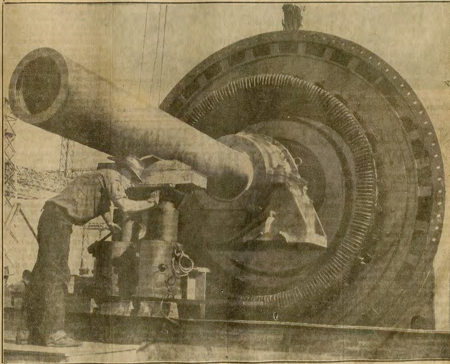
GIANT FREQUENCY CHANGER NOW NEARING COMPLETION This Might be a New Type of Coast Defense Gun, but Actually It Is a Section of a Giant Machine That Will be Used in the Peaceful Pursuit of Supplying Municipal Electricity to Los Angeles. The Machine Is Eighty Feet Long.
