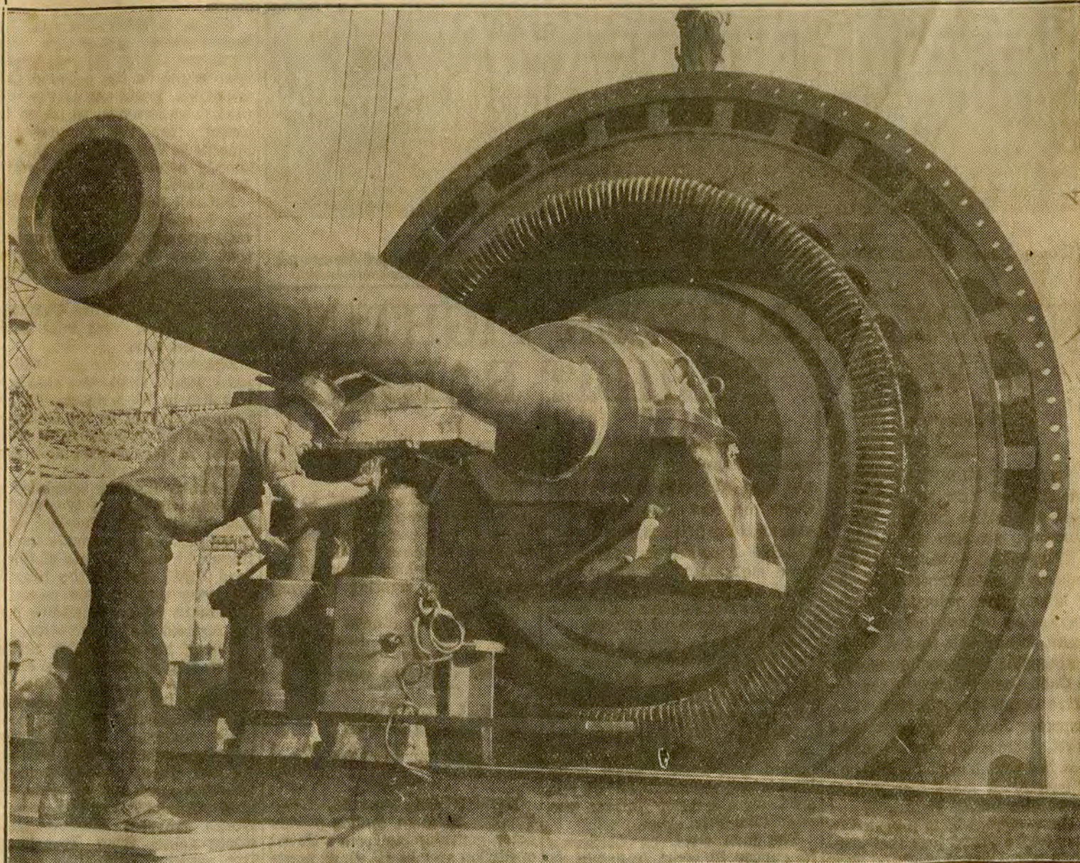
GIANT FREQUENCY CHANGER NOW NEARING COMPLETION
